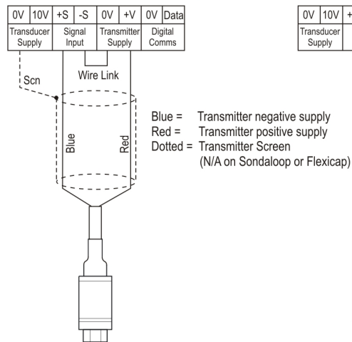
Pressure Transmitter /mA (Fig 2.3)
