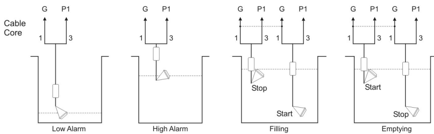
Hawker Electronics Level Controller Connections
