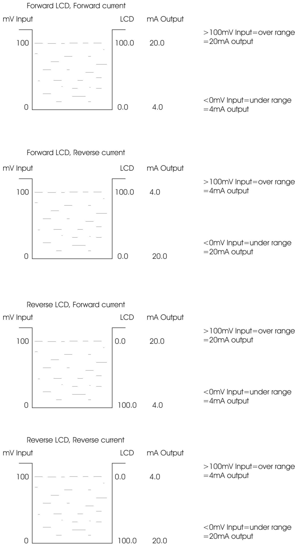
Fig 3.2 Input and output LCD/current/voltage relationship
