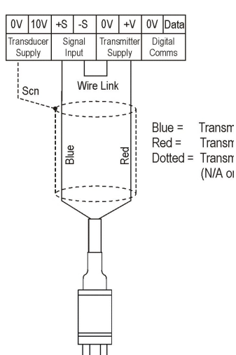
Pressure Transmitter /mA (Fig 2.3)
