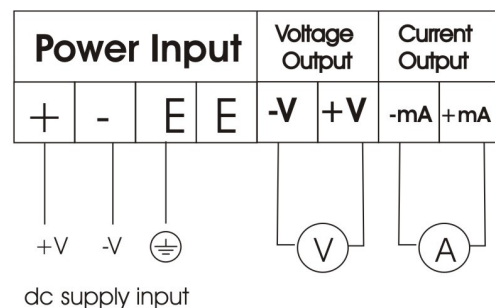
Fig 2.1(b) Power input using dc
