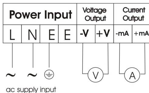
Fig 2.1(a) Power input using ac
