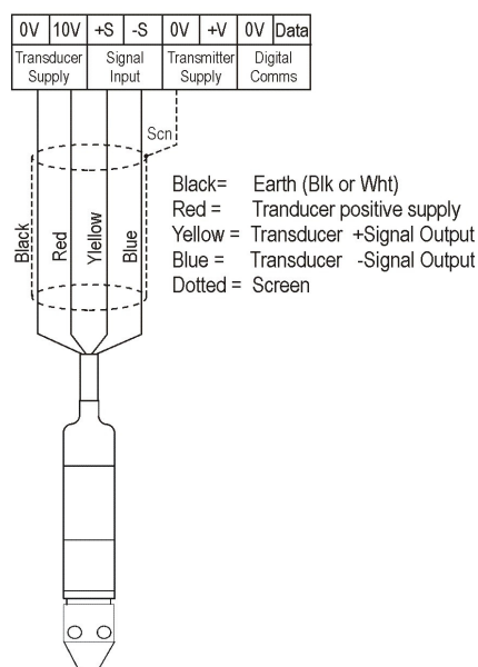
Pressure Transducer / mV Input (Fig 2.2)
