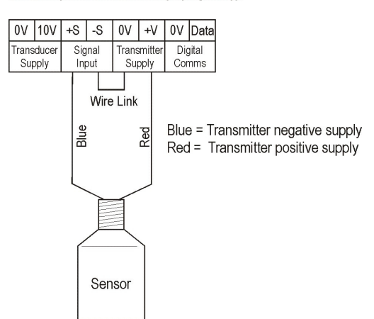
Flexicap and Sondaloop (Fig 2.5))
