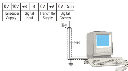
Digital Communications (Fig 2.4)
